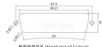
板前安装开孔 (Front Install Cutout)
