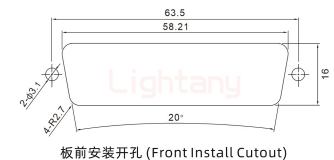
板前安装开孔 (Front Install Cutout)
